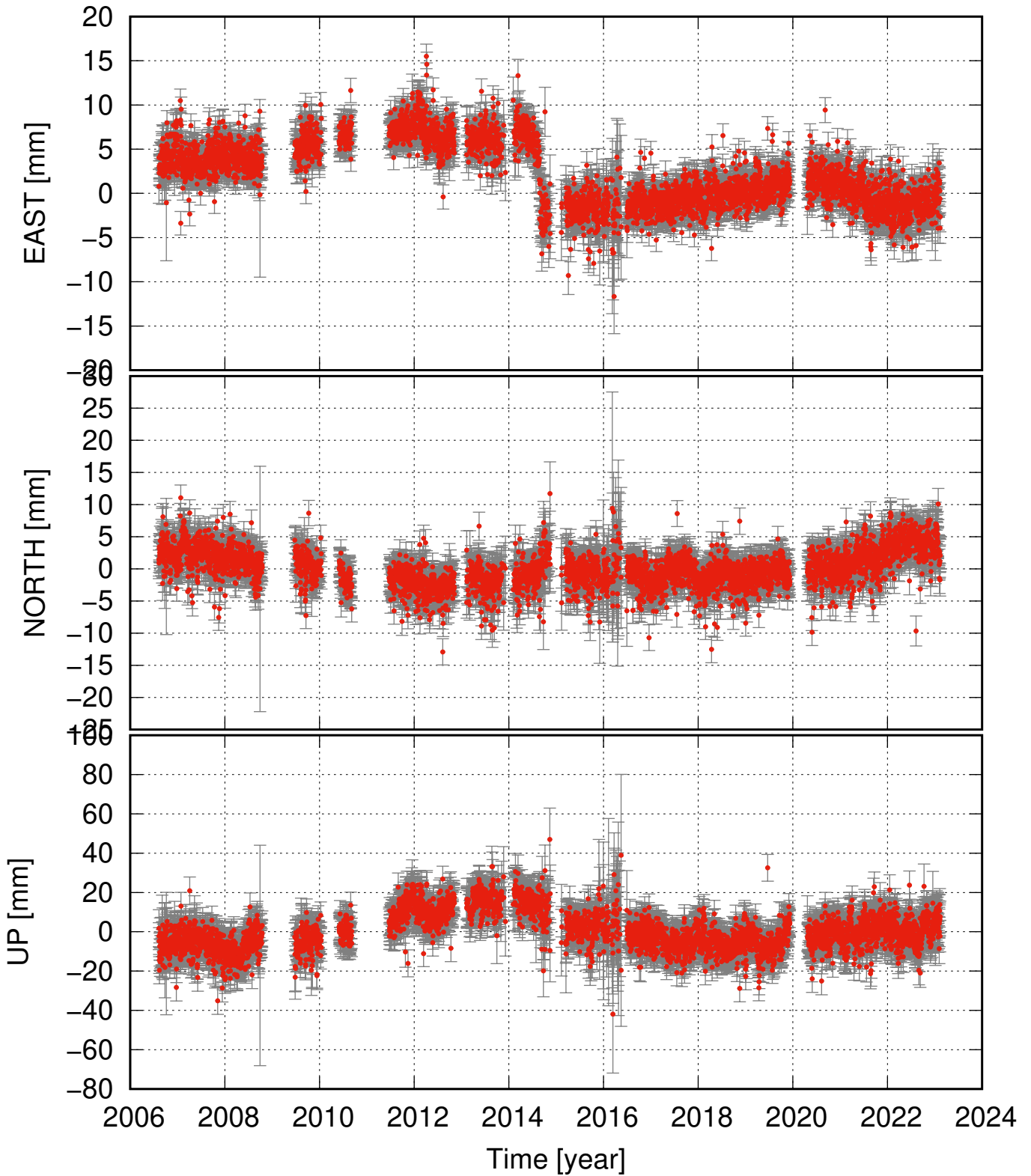
HVEL detrended and seasonal signal removed
