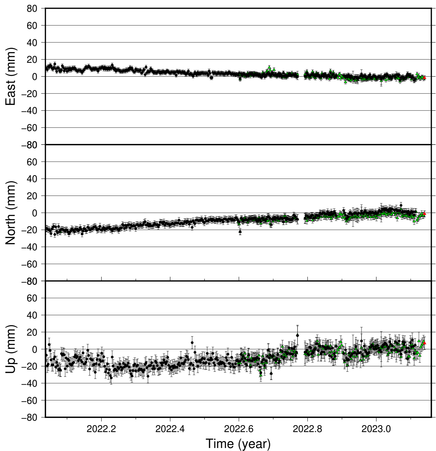
HVEL time series (IGS 2014), last 400 days
