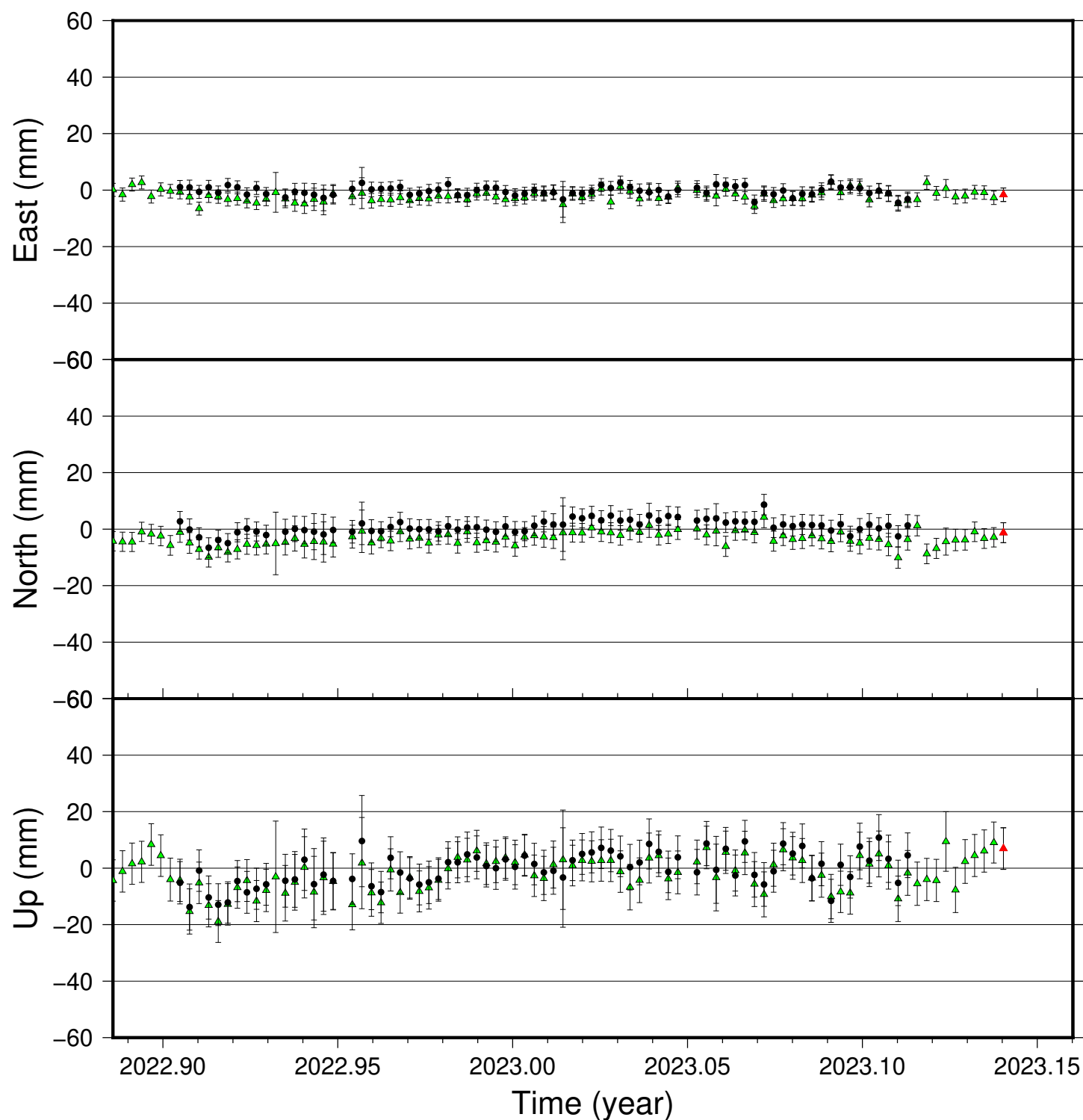
HVEL time series (IGS 2014), last 100 days
