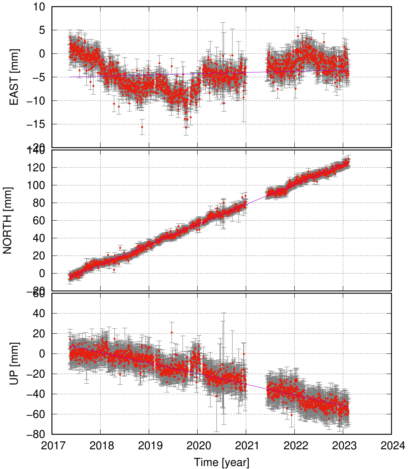
HVEH (64.01, -21.36) time series (ITRF 2014) v_e = 0.27 \pm 0.53 ; v_n = 22.72 \pm 0.42 ; v_u = -10.57 \pm 1.04 mm/yr
