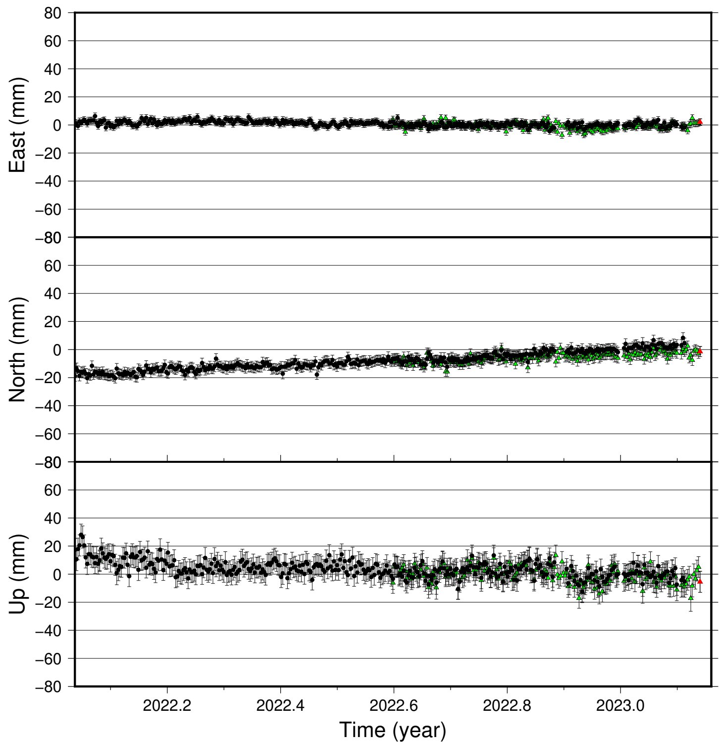
HVEH time series (IGS 2014), last 400 days
