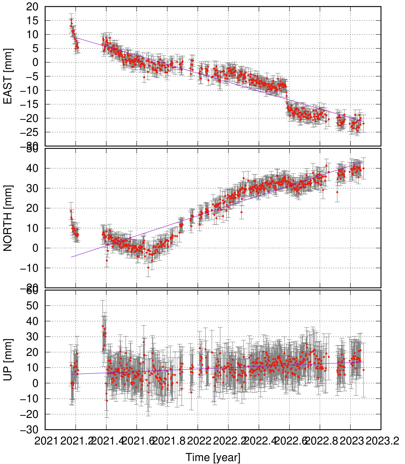
HVAS (64.02, -22.13) time series (ITRF 2014) v_e = -15.96 \pm 1.52 ; v_n = 25.09 \pm 2.84 ; v_u = 4.15 \pm 3.08 mm/yr
