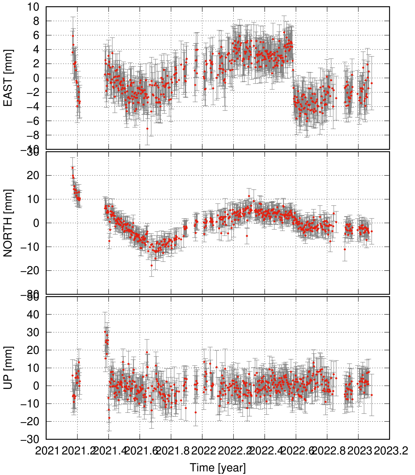
HVAS residual time series
