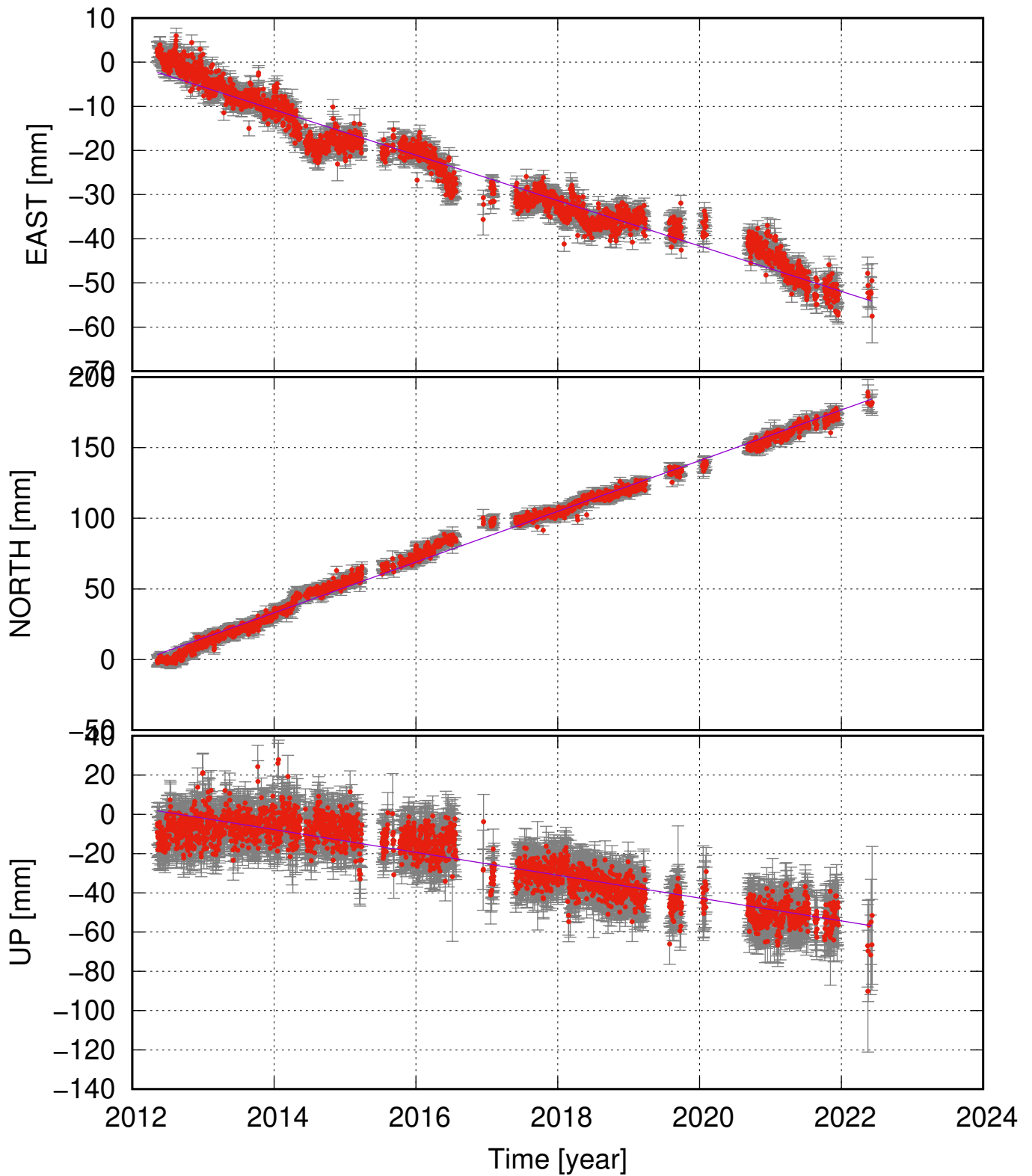
HUSM (64.07, -21.42) time series (ITRF 2014) v_e = -5.14 \pm 0.28 ; v_n = 17.94 \pm 0.41 ; v_u = -5.80 \pm 0.72 mm/yr
