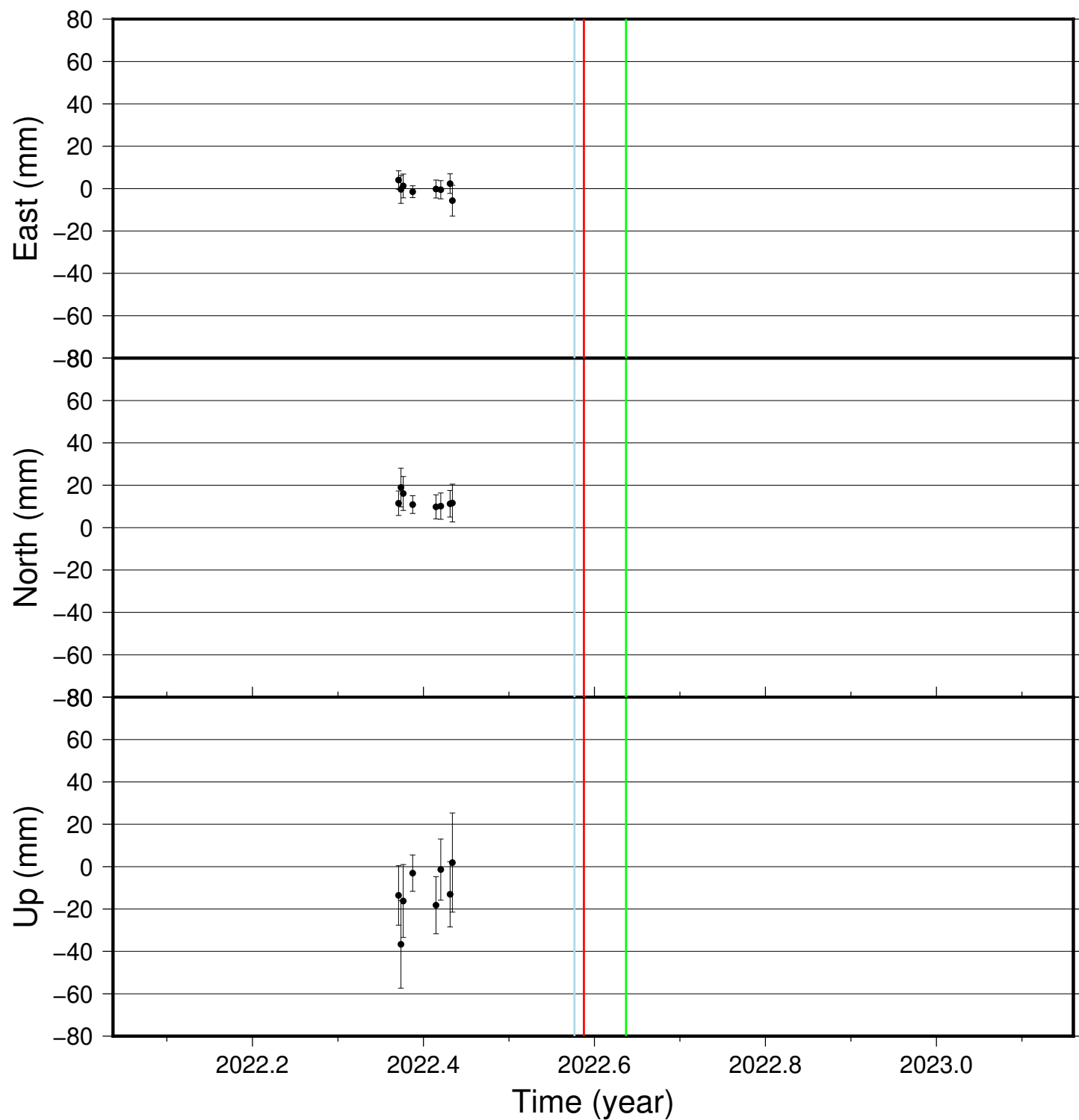
HUSM time series (IGS 2014), last 400 days
