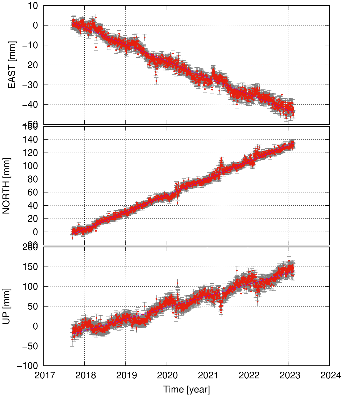
HSKC (64.62, -18.08) time series (ITRF 2014) v_e = -8.34 \pm 0.38 ; v_n = 25.49 \pm 0.63 ; v_u = 29.19 \pm 2.05 mm/yr
