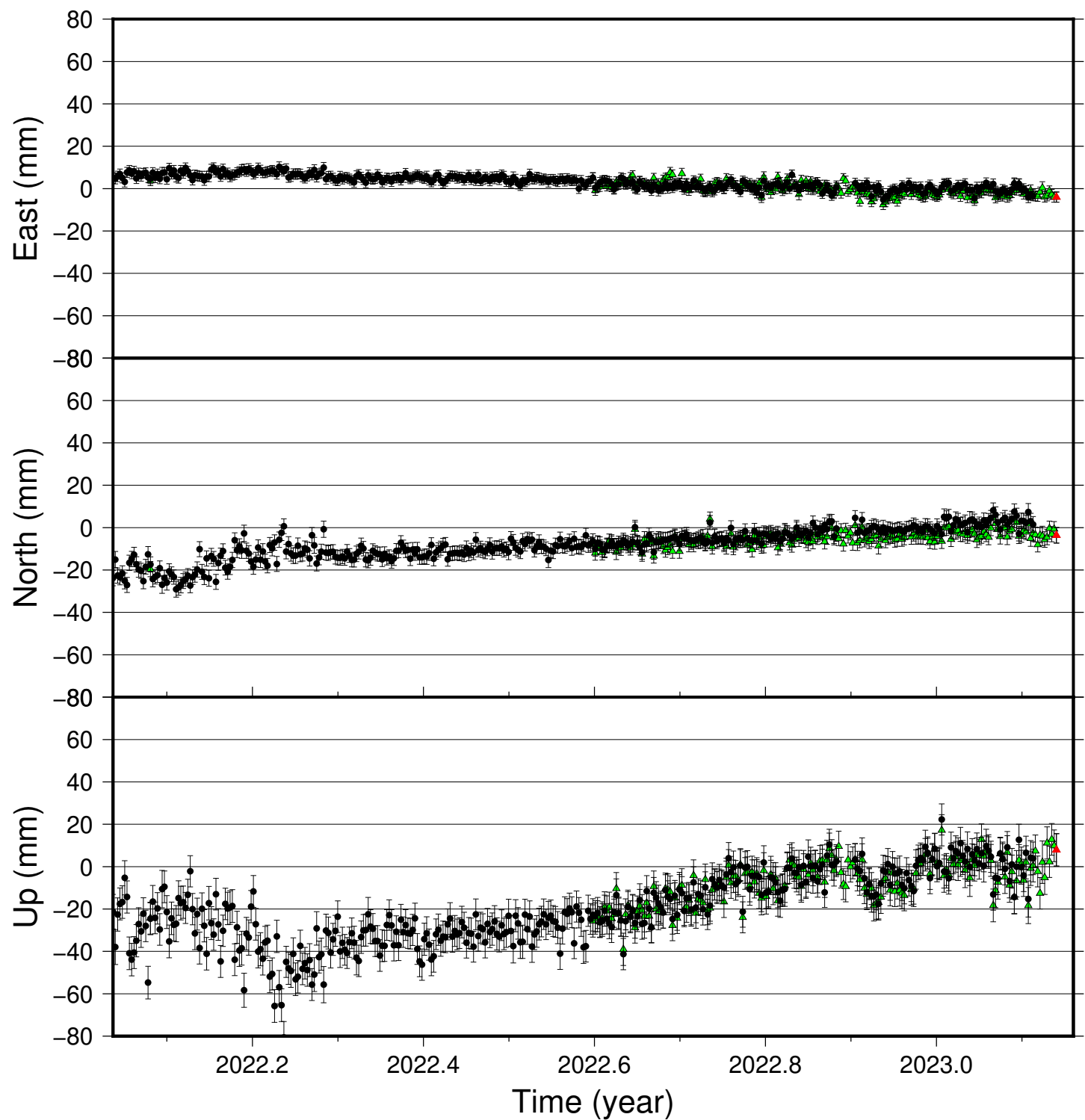
HSKC time series (IGS 2014), last 400 days
