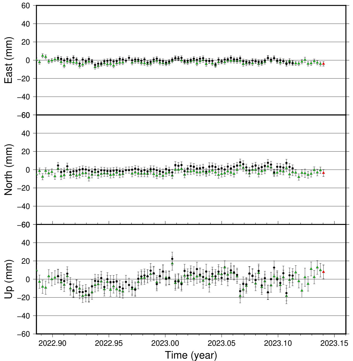
HSKC time series (IGS 2014), last 100 days
