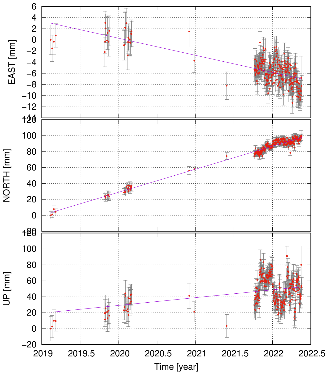
HRIC (64.95, -16.92) time series (ITRF 2014) v_e = -3.06 \pm 0.58 ; v_n = 28.91 \pm 1.04 ; v_u = 9.77 \pm 5.06 mm/yr
