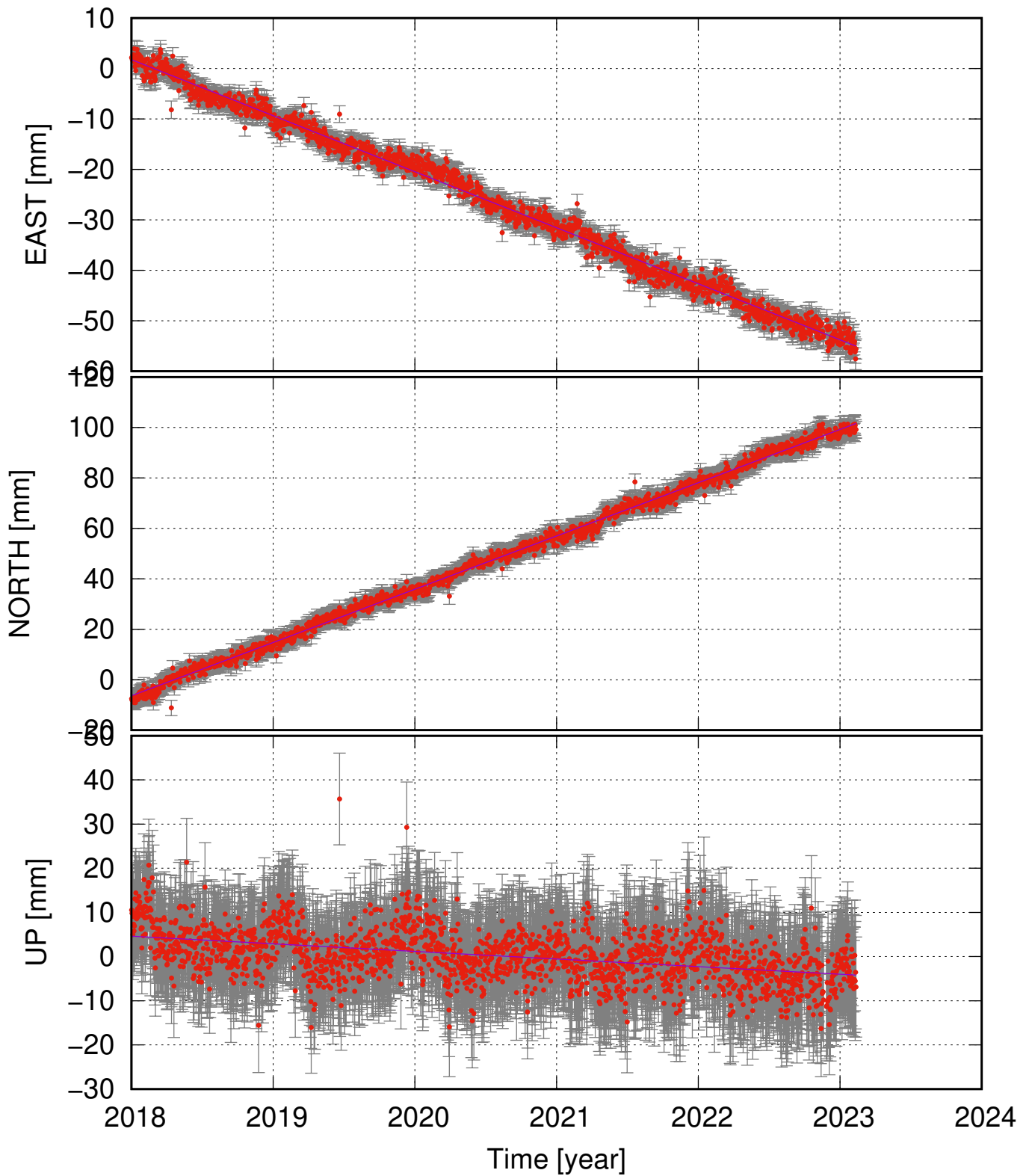
HRAC (66.11, -20.12) time series (ITRF 2014) v_e = -11.11 \pm 0.29 ; v_n = 21.11 \pm 0.33 ; v_u = -1.72 \pm 0.98 mm/yr
