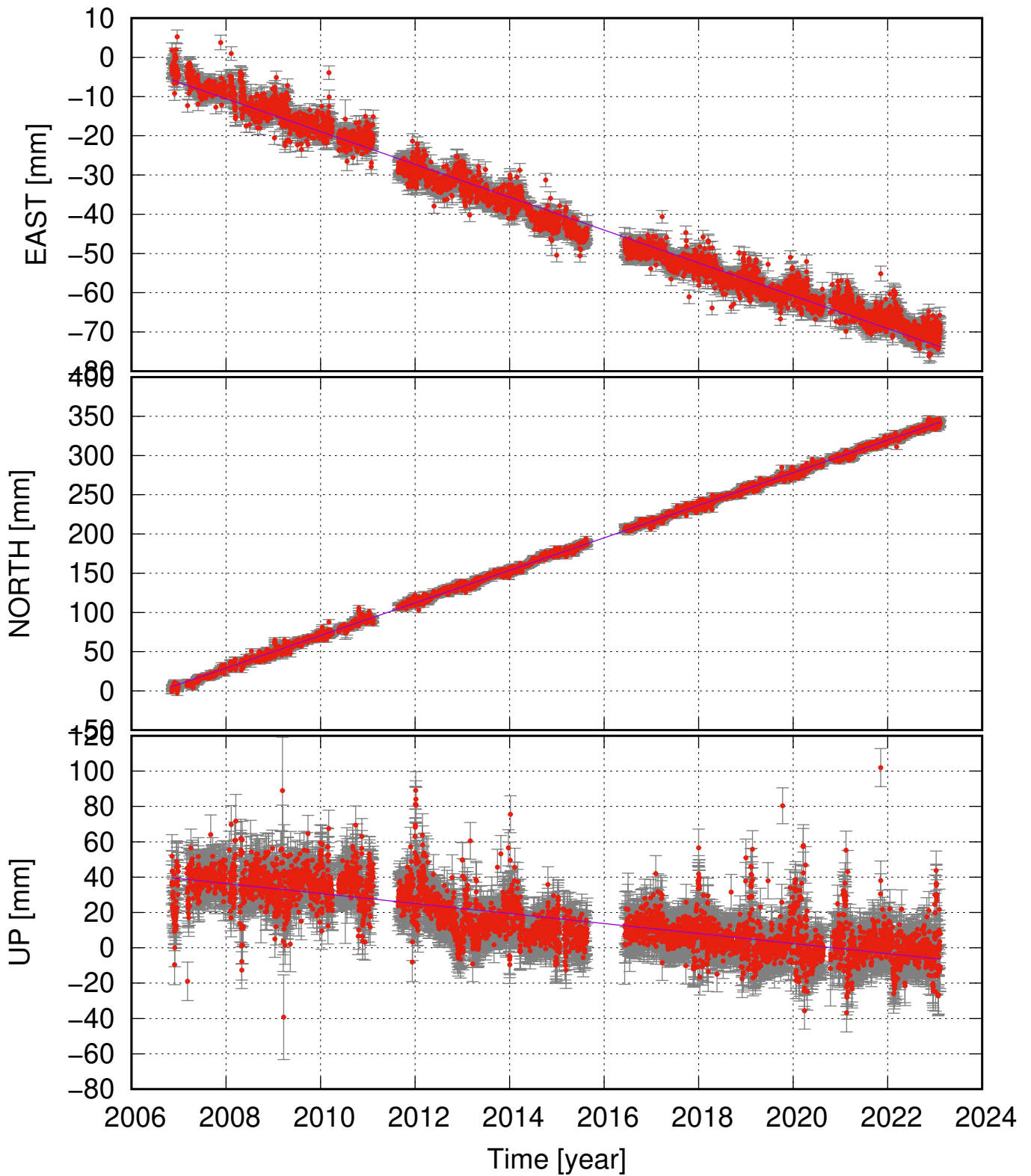
HOTJ (66.16, -17.24) time series (ITRF 2014) v_e = -4.19 \pm 0.16 ; v_n = 20.73 \pm 0.17 ; v_u = -2.83 \pm 0.66 mm/yr
