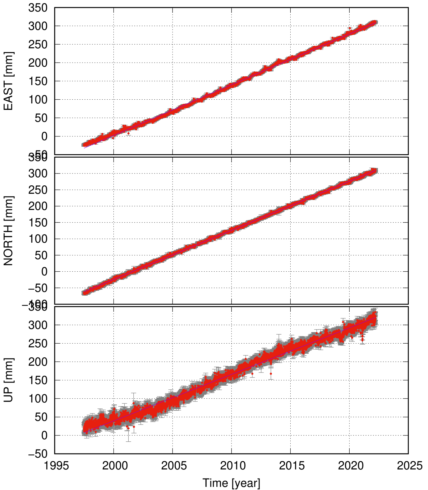
HOFN (64.27, -15.20) time series (ITRF 2014) v_e = 13.78 \pm 0.16 ; v_n = 15.01 \pm 0.09 ; v_u = 12.66 \pm 0.38 mm/yr
