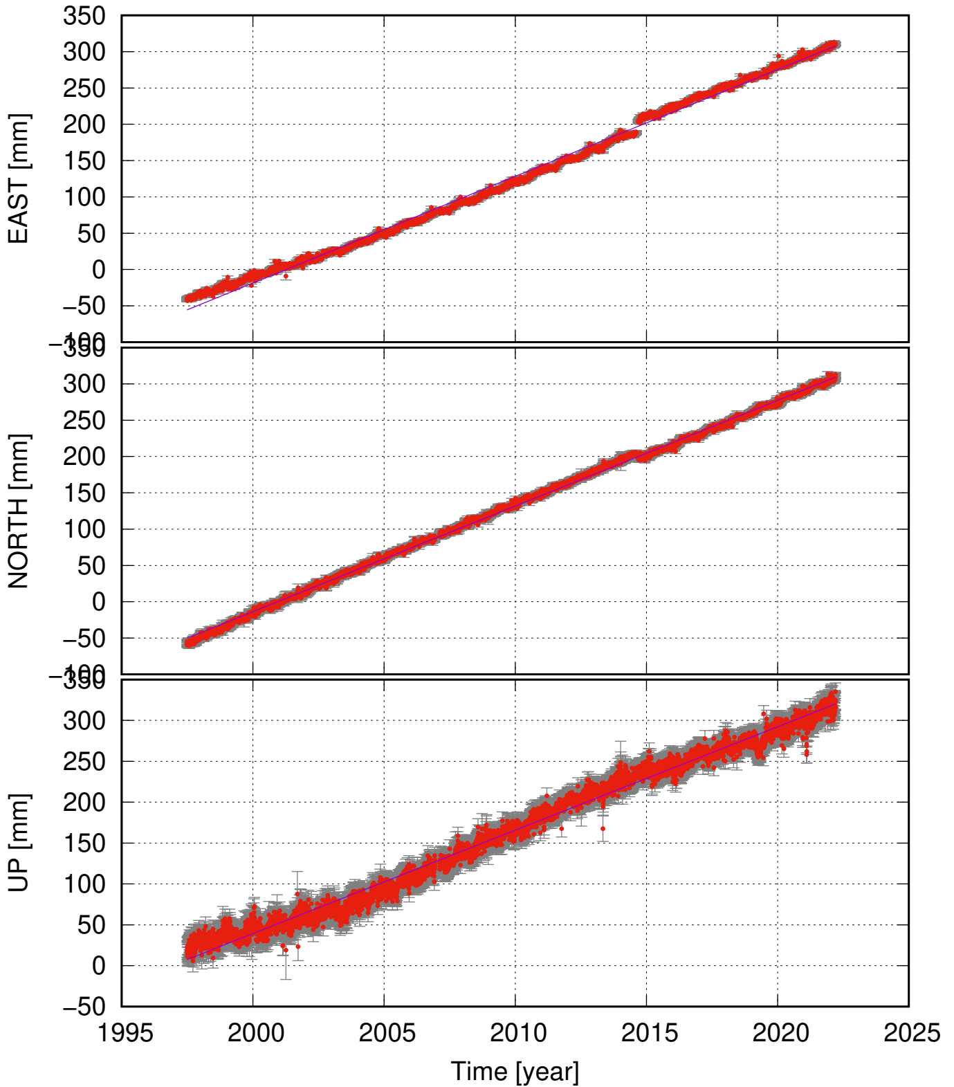
HOFN (64.27, -15.20) time series (ITRF 2014) v_e = 14.71 \pm 0.28 ; v_n = 14.54 \pm 0.15 ; v_u = 12.66 \pm 0.38 mm/yr
