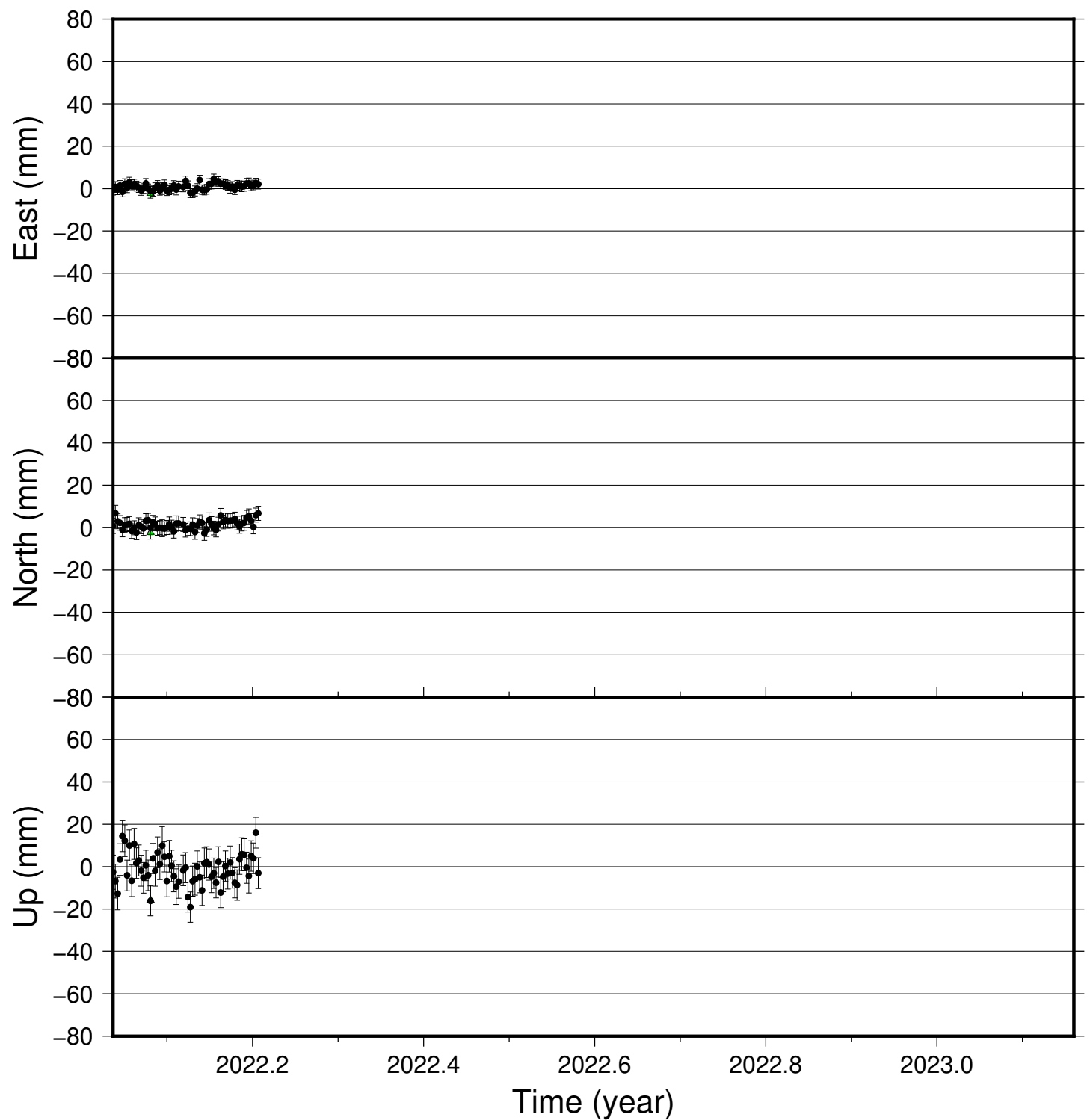
HOFN time series (IGS 2014), last 400 days
