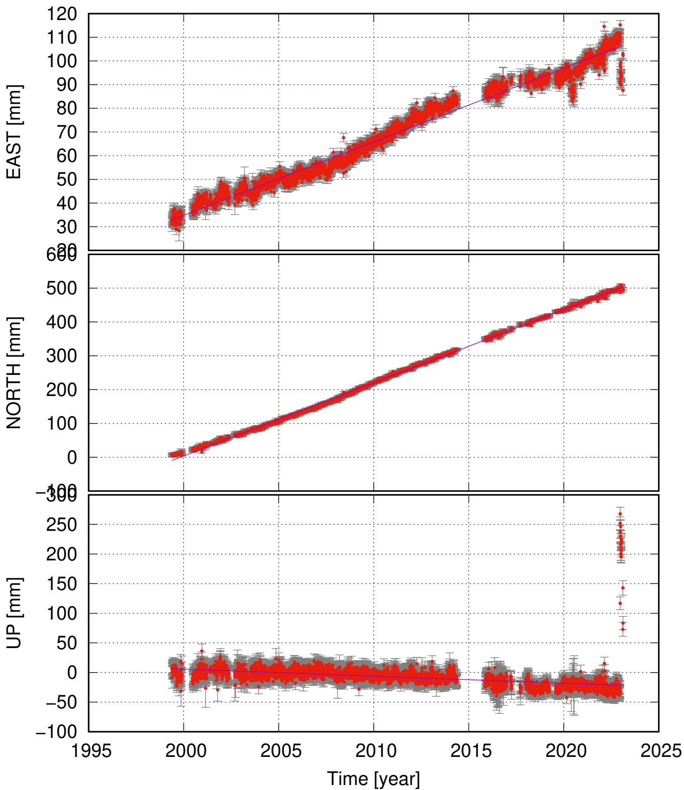
HLID (63.92, -21.39) time series (ITRF 2014) v_e = 3.11 \pm 0.13 ; v_n = 21.63 \pm 0.19 ; v_u = -1.19 \pm 0.68 mm/yr
