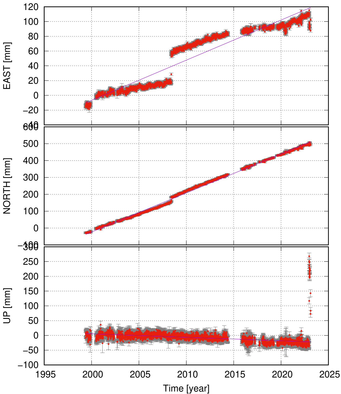
HLID (63.92, -21.39) time series (ITRF 2014) v_e = 5.44 \pm 0.53 ; v_n = 23.14 \pm 0.41 ; v_u = -1.19 \pm 0.68 mm/yr
