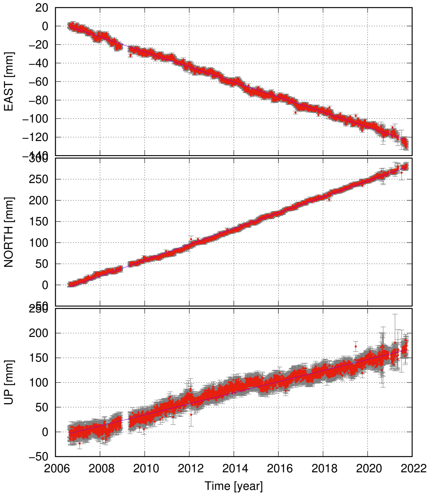
HLFJ (64.28, -20.14) time series (ITRF 2014) v_e = -8.11 \pm 0.15 ; v_n = 18.72 \pm 0.23 ; v_u = 11.20 \pm 0.54 mm/yr
