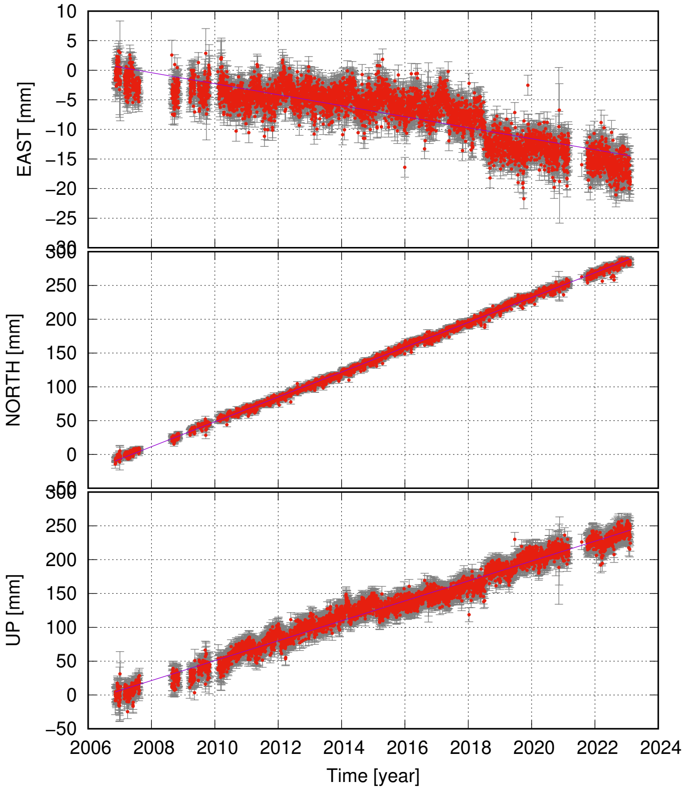
HESA (64.05, -19.56) time series (ITRF 2014) v_e = -0.93 \pm 0.15 ; v_n = 18.39 \pm 0.19 ; v_u = 14.71 \pm 0.58 mm/yr
