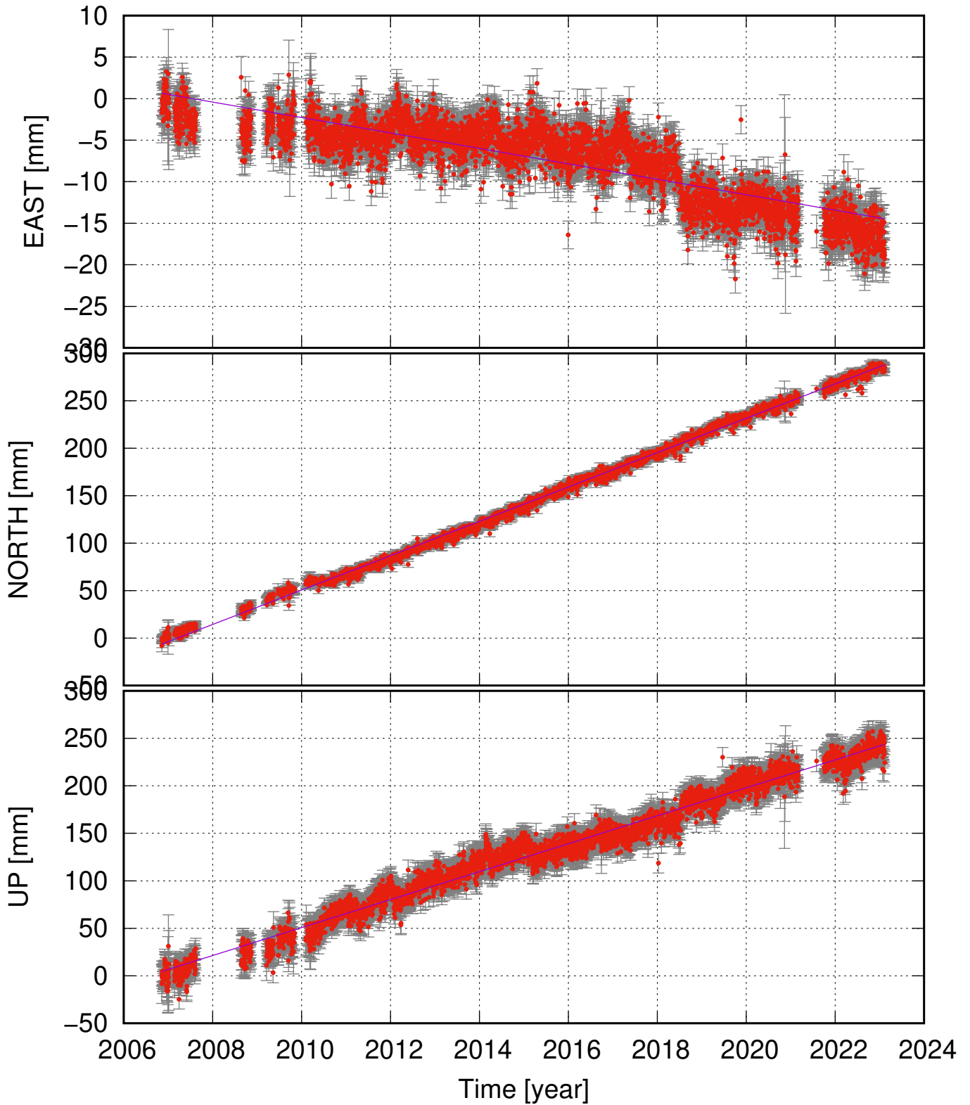
HESA (64.05, -19.56) time series (ITRF 2014) v_e = -0.93 \pm 0.15 ; v_n = 18.10 \pm 0.23 ; v_u = 14.71 \pm 0.58 mm/yr
