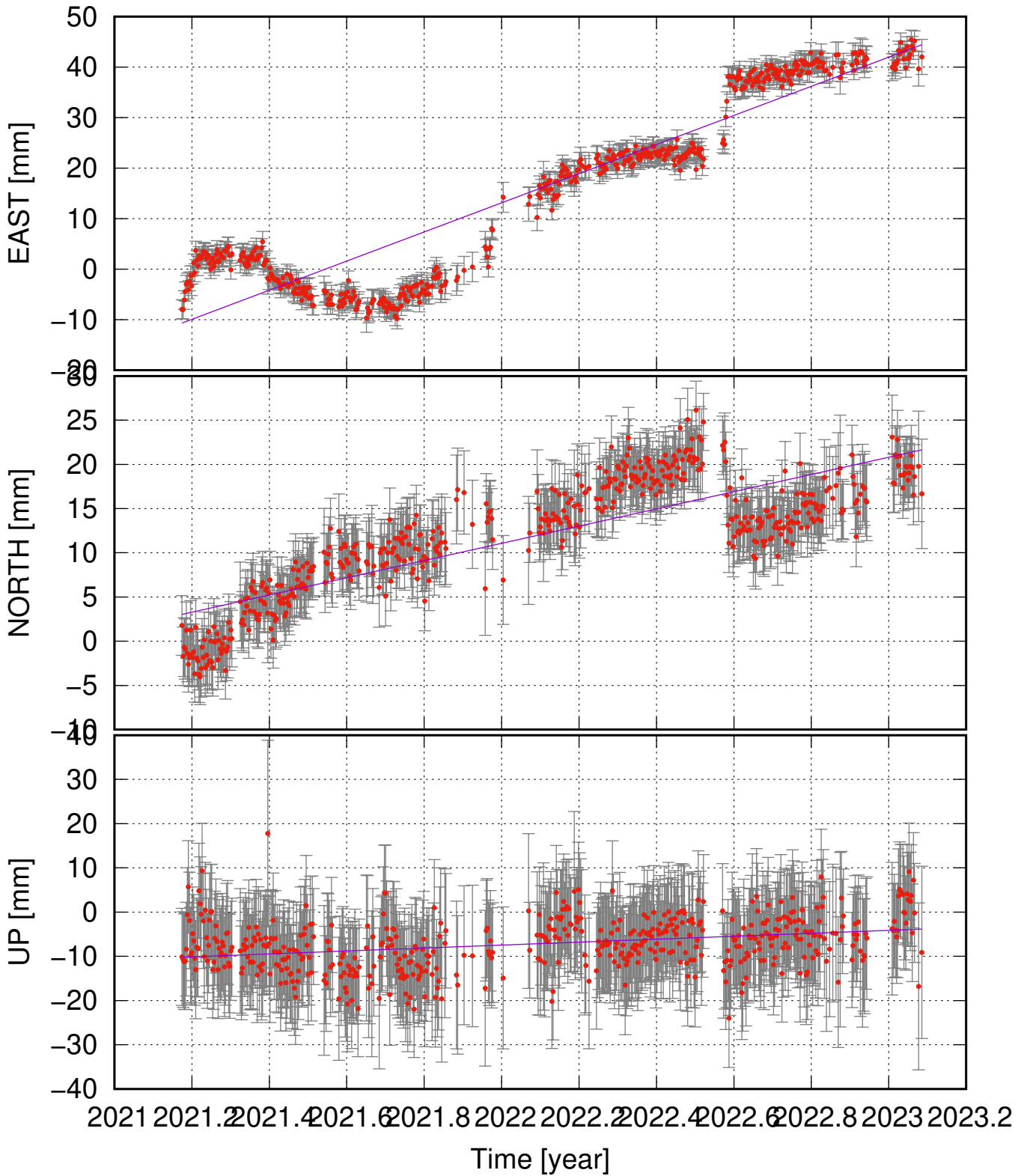
HERV (63.87, -21.88) time series (ITRF 2014) v_e = 28.84 \pm 3.41 ; v_n = 9.73 \pm 1.98 ; v_u = 3.33 \pm 2.87 mm/yr
