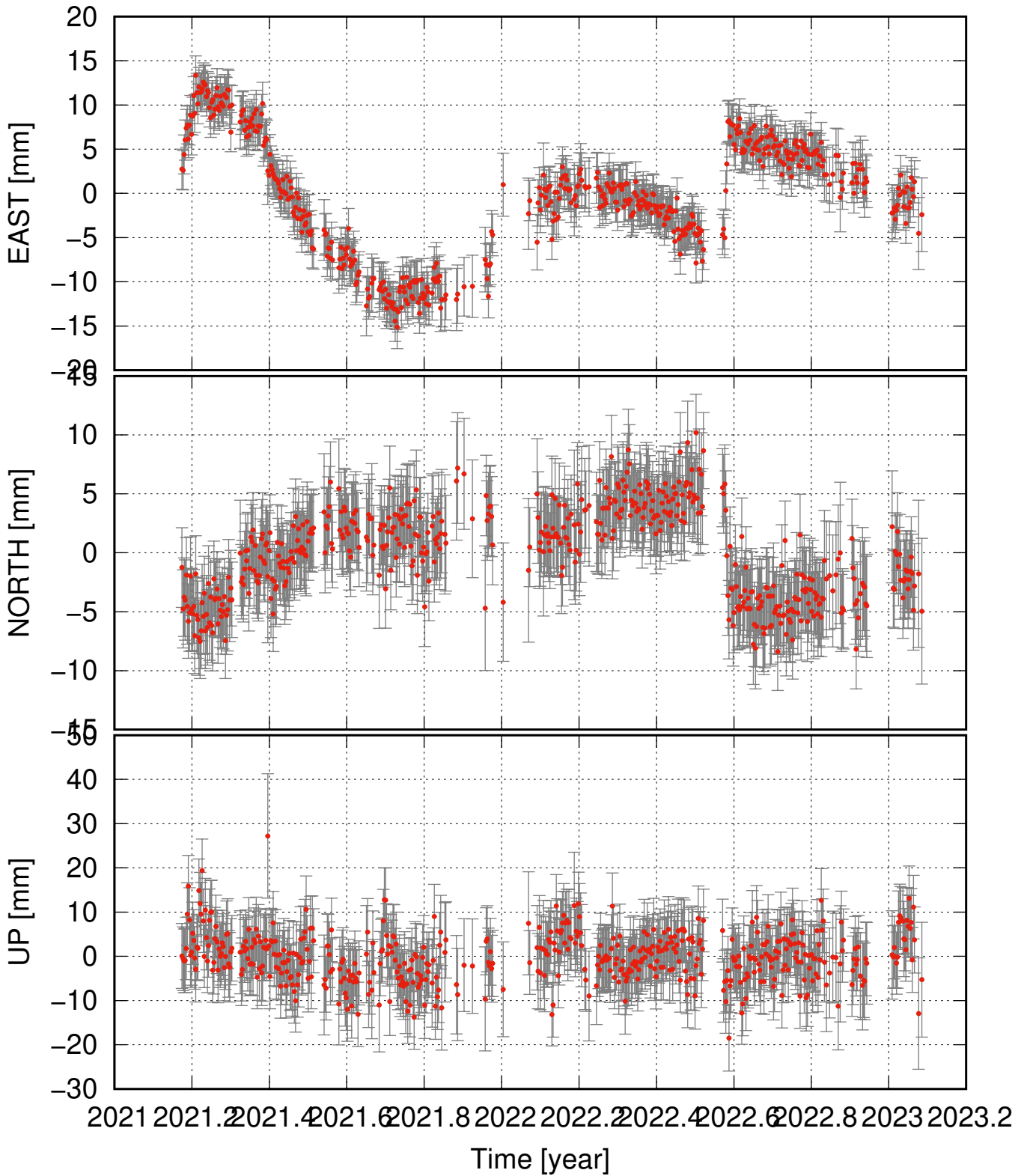
HERV residual time series (some major events removed as well)
