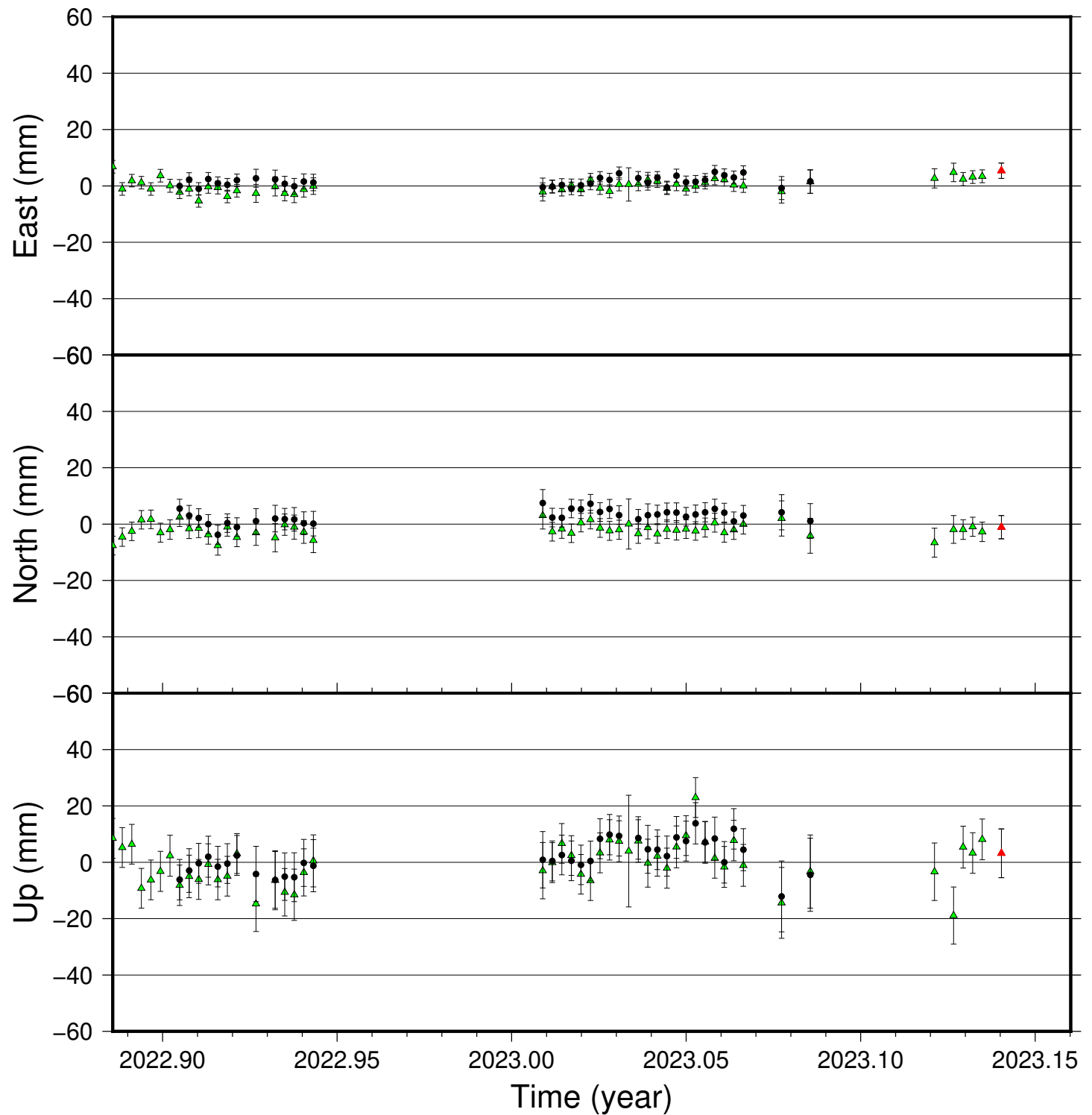
HERV time series (IGS 2014), last 100 days
