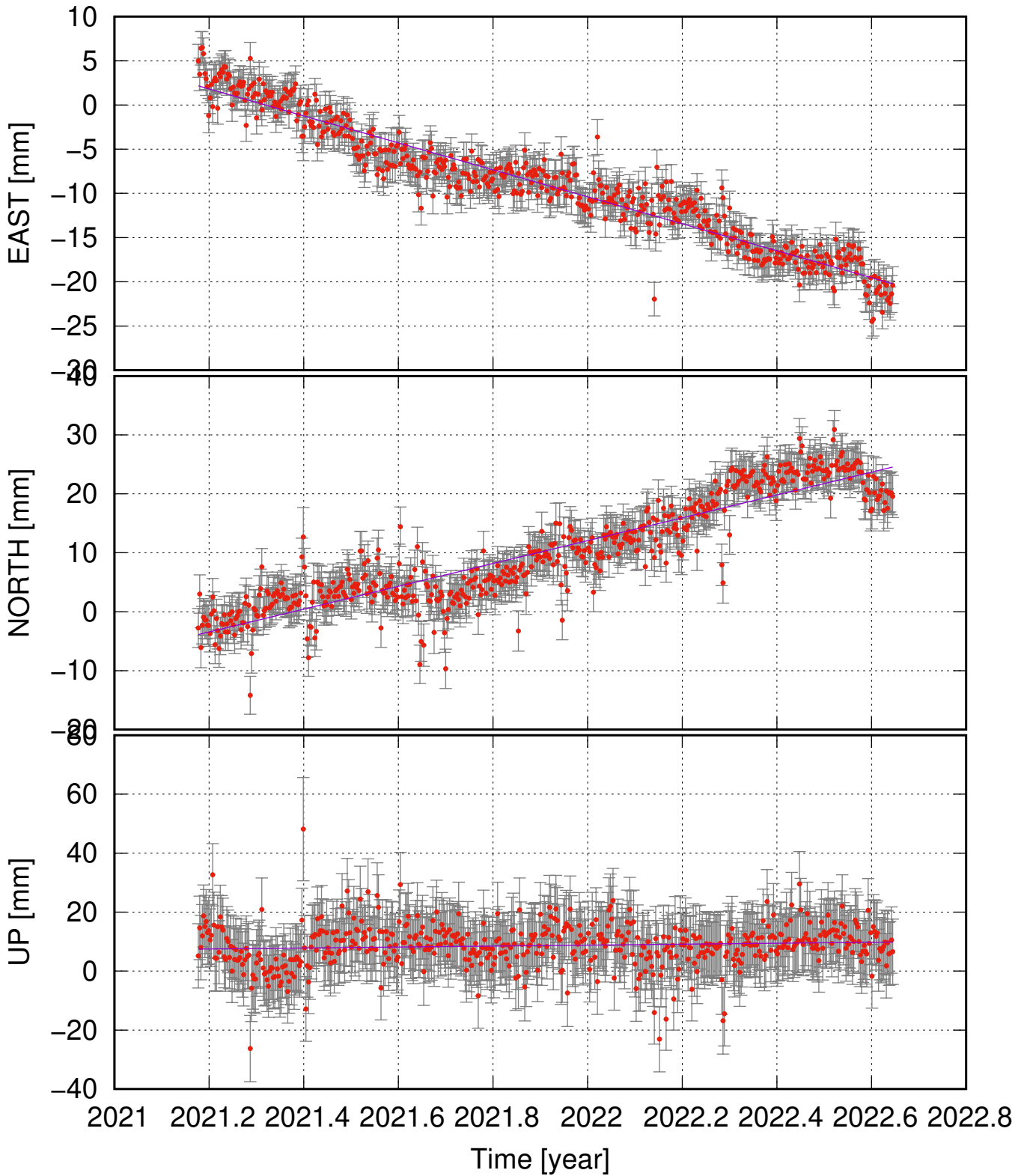
HEL (64.02, -21.85) time series (ITRF 2014) v_e = -15.26 \pm 1.28 ; v_n = 19.38 \pm 2.53 ; v_u = 1.61 \pm 4.84 mm/yr
