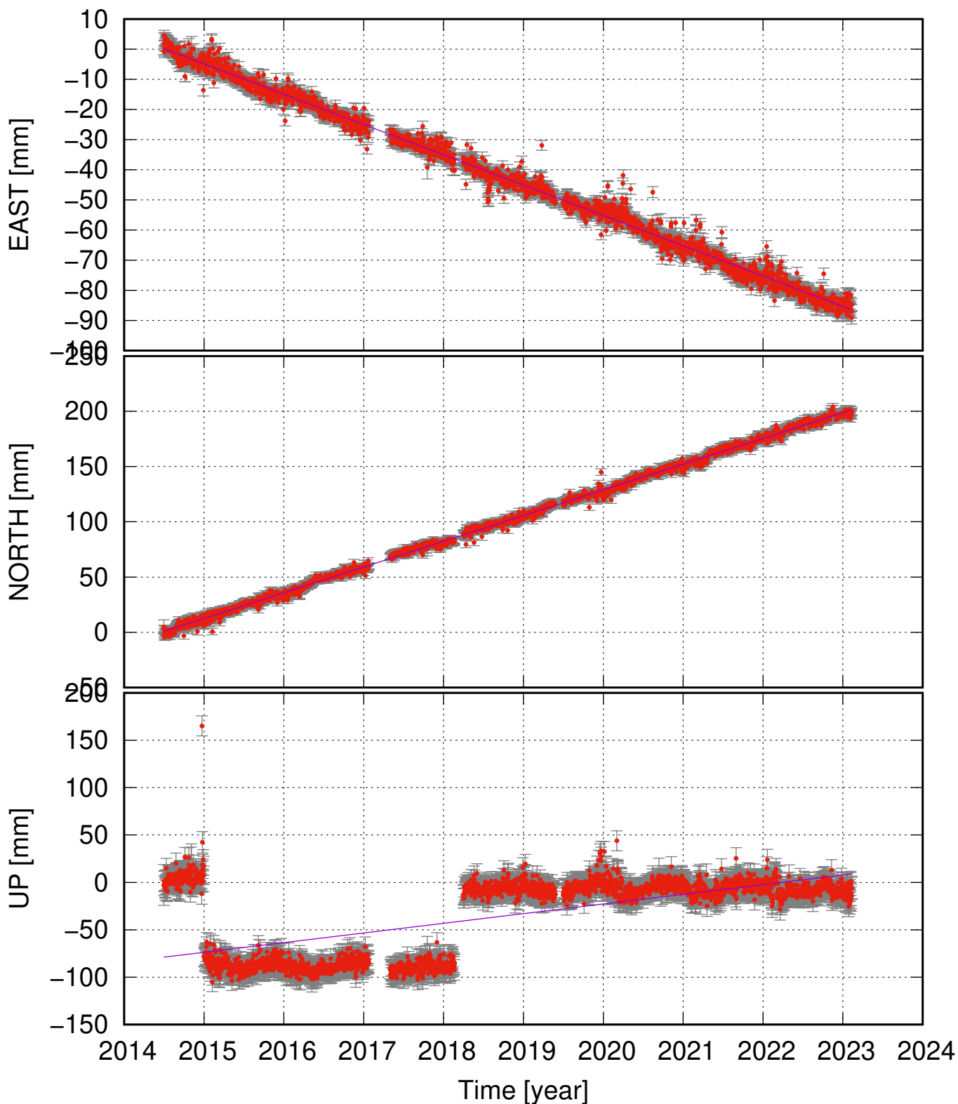
HELC (65.94, -18.39) time series (ITRF 2014) v_e = -10.06 \pm 0.24 ; v_n = 23.28 \pm 0.27 ; v_u = 10.20 \pm 3.66 mm/yr
