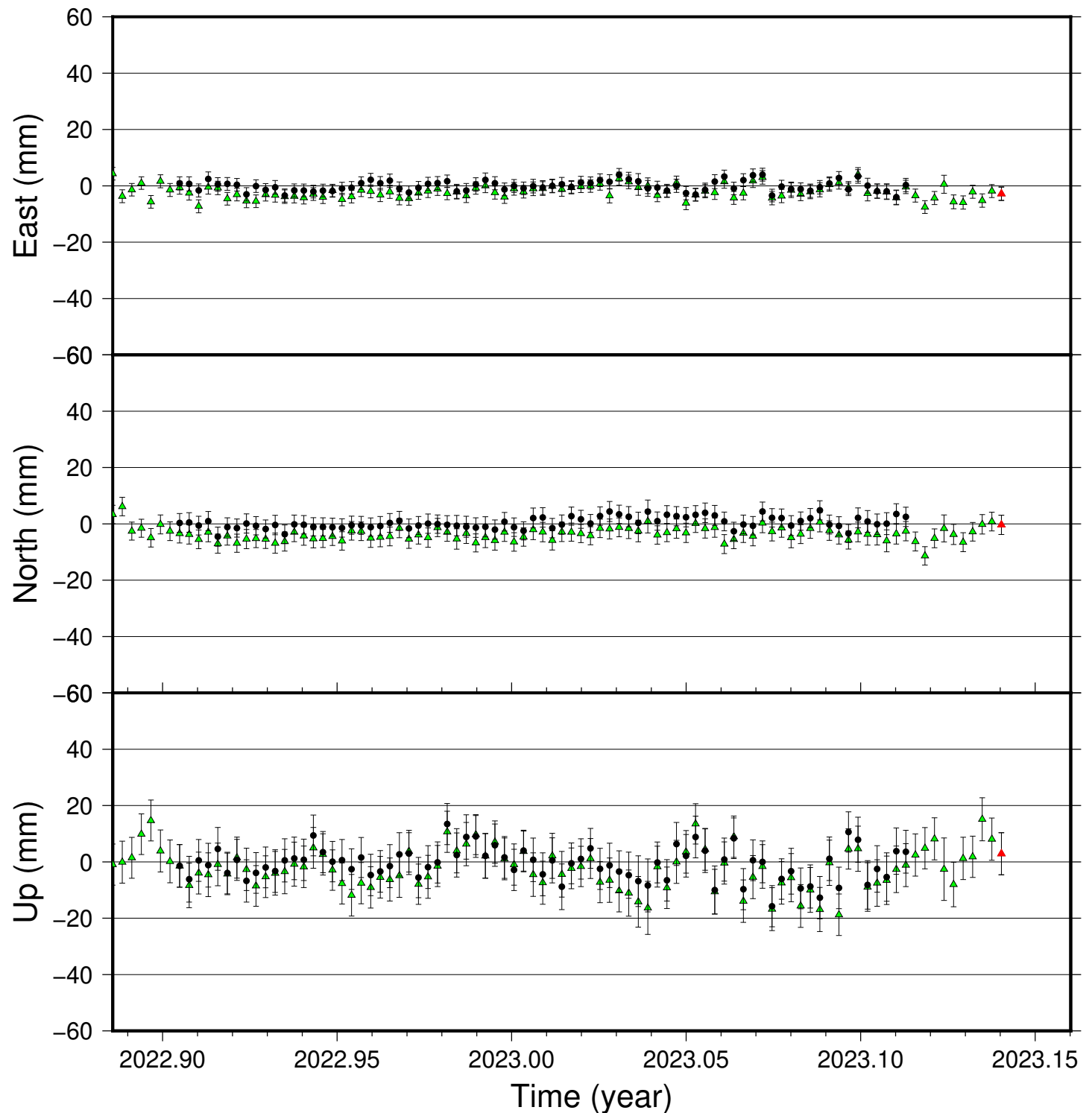
HELC time series (IGS 2014), last 100 days
