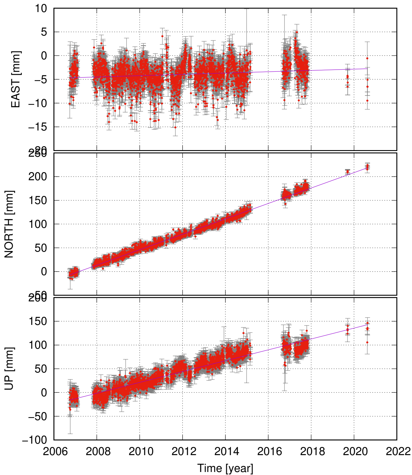
HEKR (64.01, -19.66) time series (ITRF 2014) v_e = 0.14 \pm 0.17 ; v_n = 16.24 \pm 0.33 ; v_u = 11.43 \pm 0.77 mm/yr
