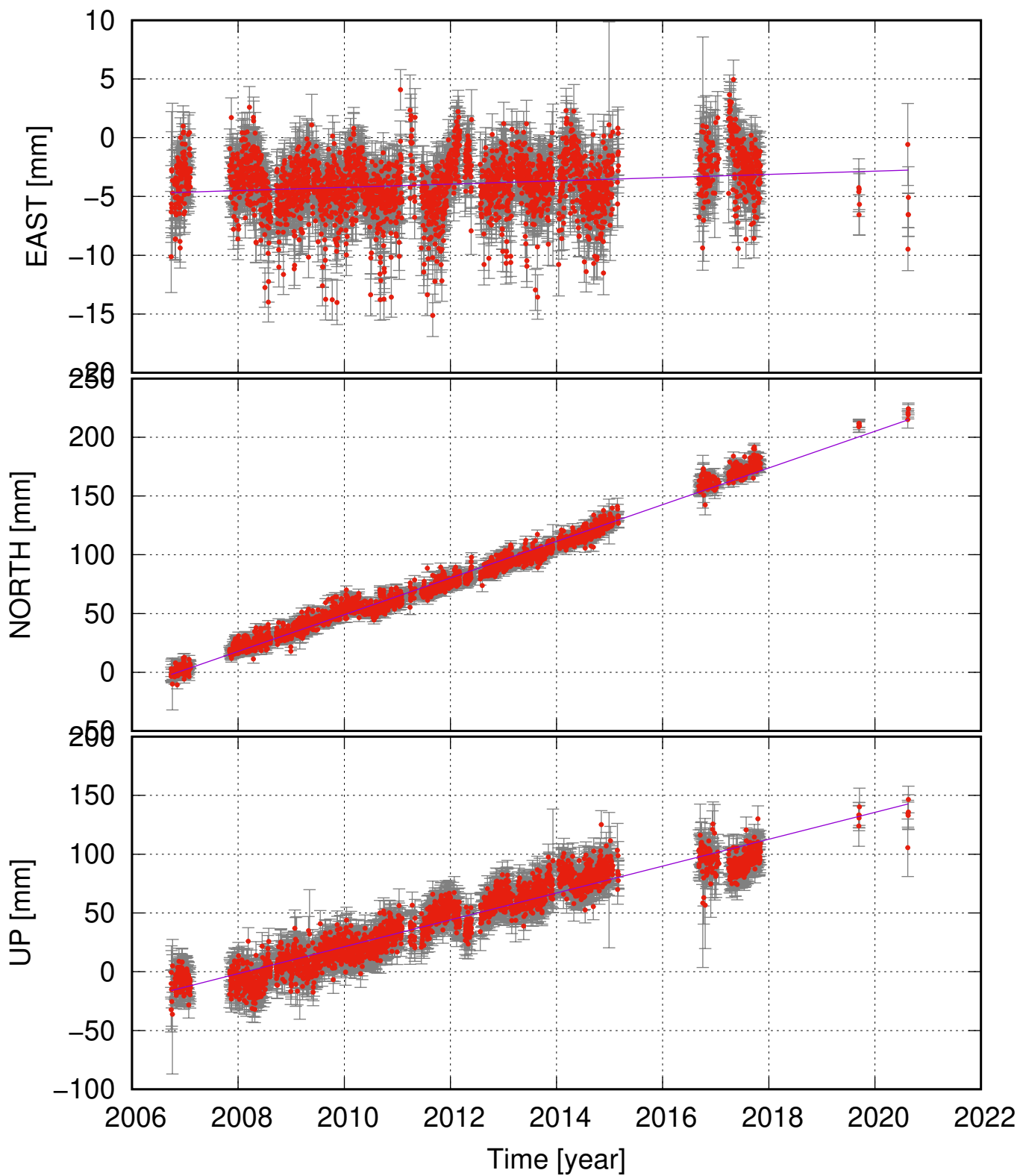
HEKR (64.01, -19.66) time series (ITRF 2014) ve = 0.14 \pm 0.17 ; vn = 15.60 \pm 0.39 ; vu = 11.43 \pm 0.77 mm/yr
