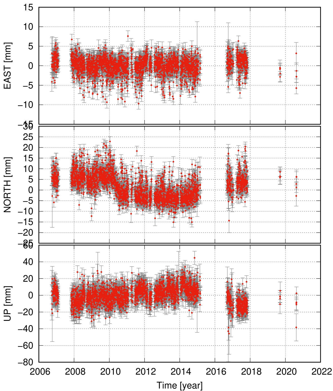
HEKR detrended and seasonal signal removed
