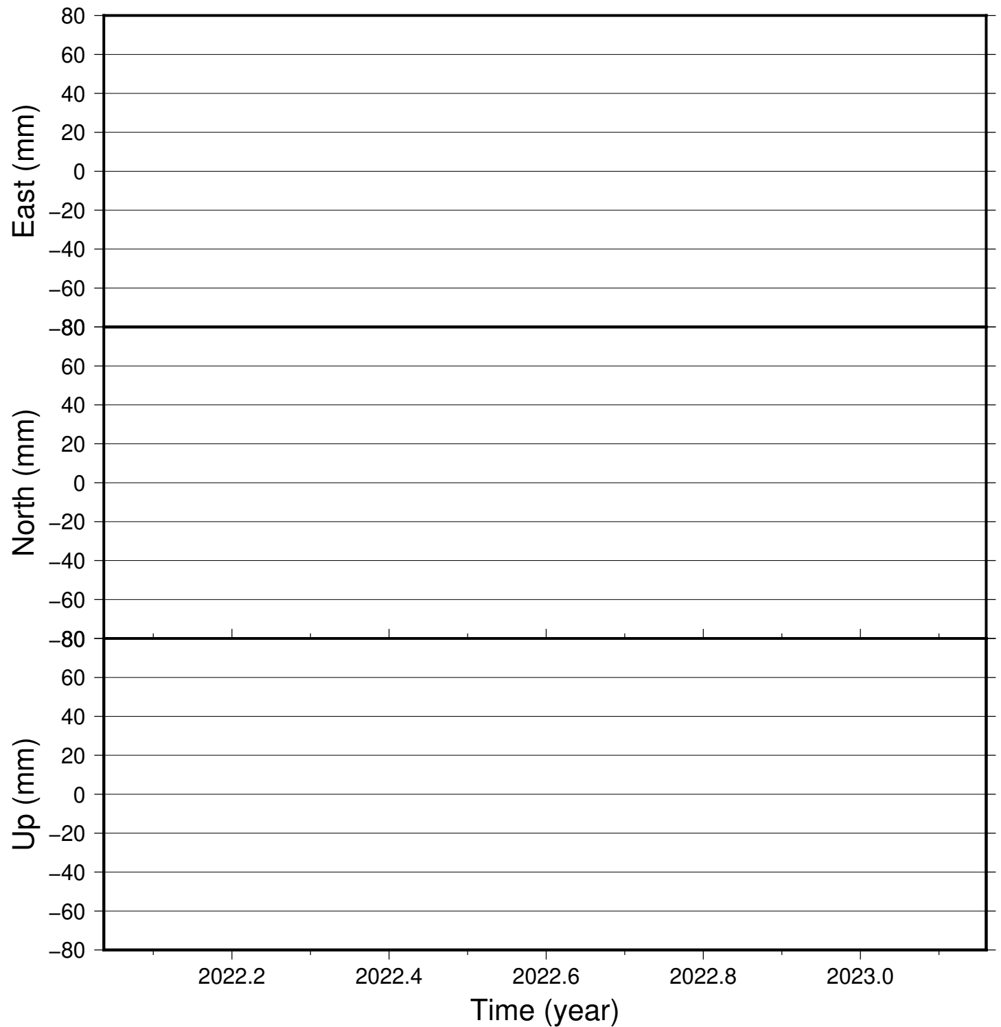
HEKR time series (IGS 2014), last 400 days
