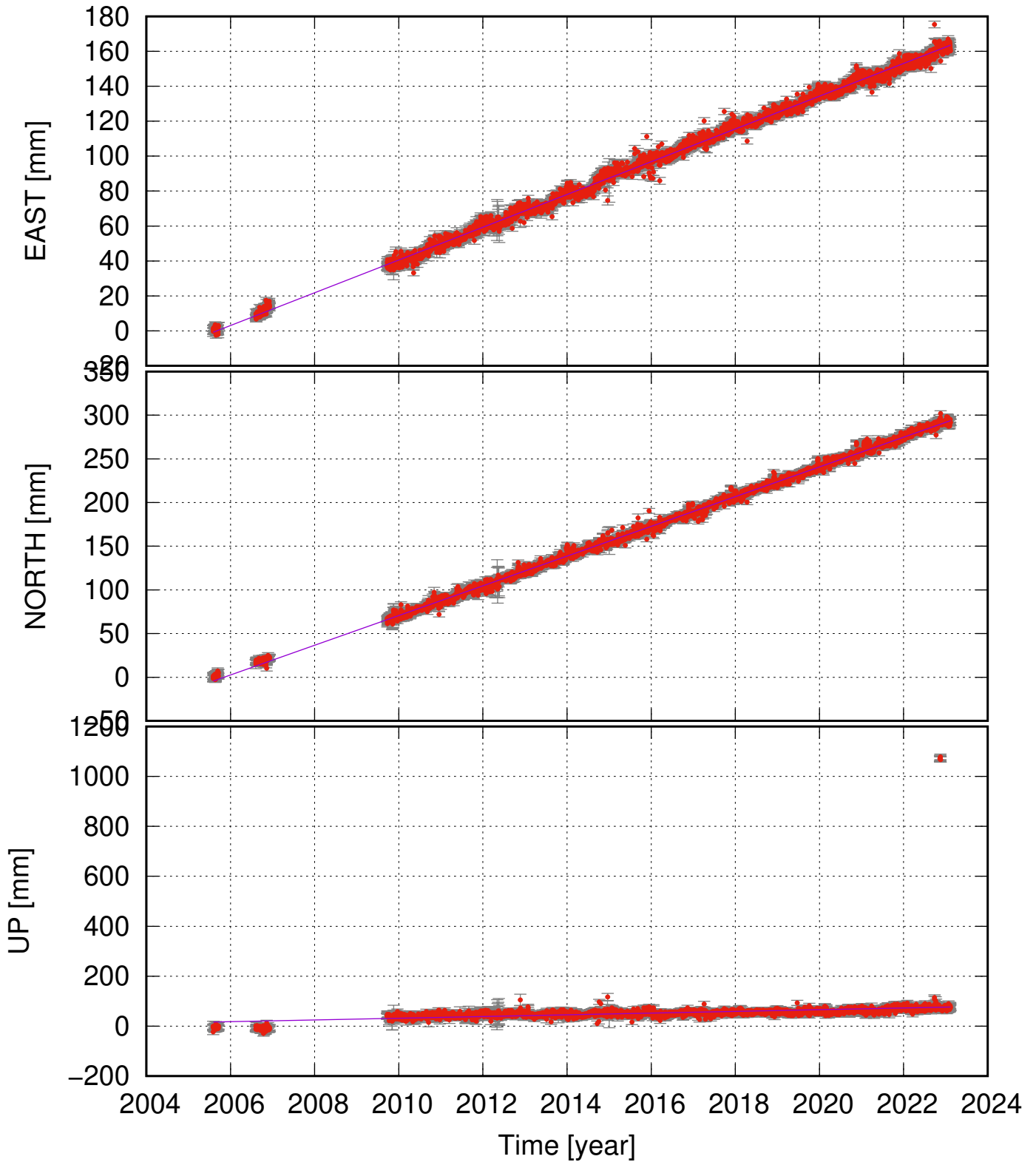
HEID (65.38, -14.54) time series (ITRF 2014) v_e = 9.37 \pm 0.13 ; v_n = 17.02 \pm 0.16 ; v_u = 3.45 \pm 2.07 mm/yr
