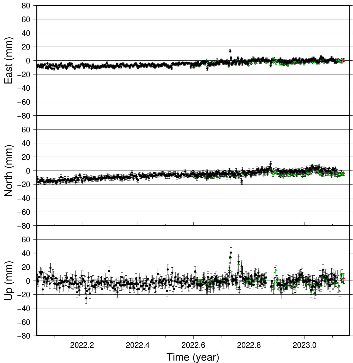
HEID time series (IGS 2014), last 400 days
