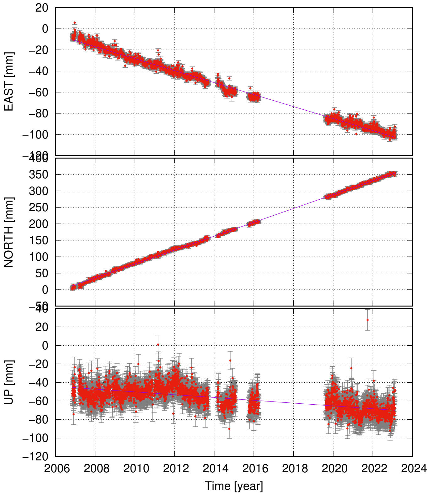
HEDI (66.08, -17.31) time series (ITRF 2014) v_e = -5.66 \pm 0.16 ; v_n = 21.07 \pm 0.18 ; v_u = -1.52 \pm 0.51 mm/yr
