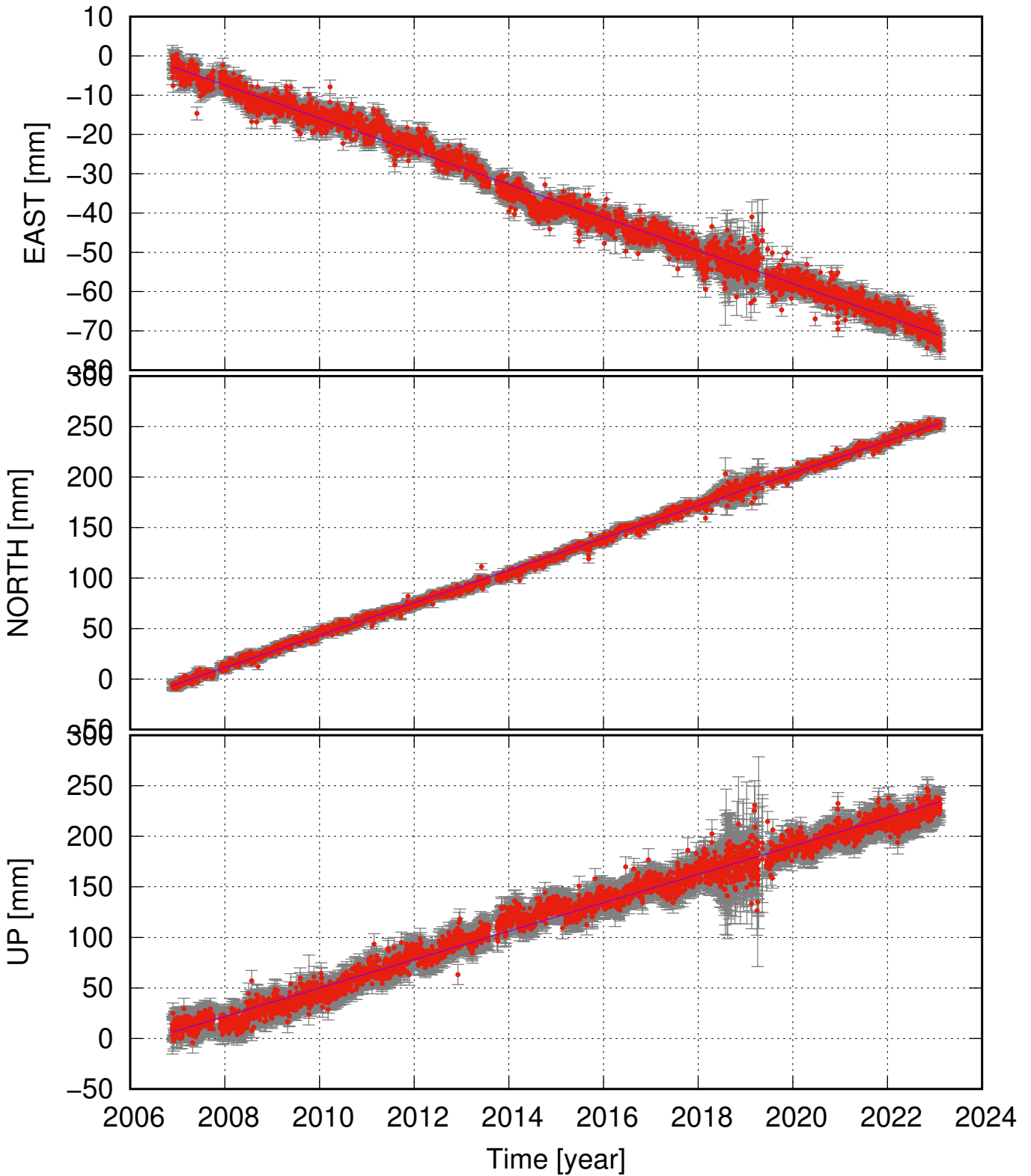
HAUD (63.97, -19.96) time series (ITRF 2014) v_e = -4.21 \pm 0.13 ; v_n = 16.02 \pm 0.17 ; v_u = 14.04 \pm 0.49 mm/yr
