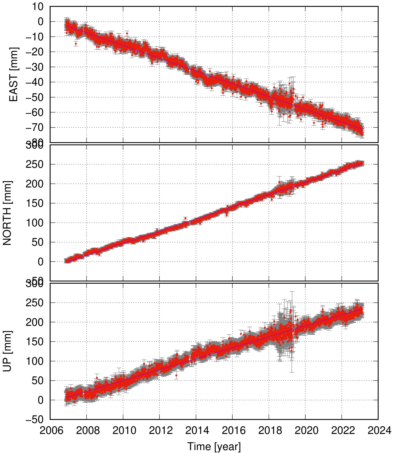
HAUD (63.97, -19.96) time series (ITRF 2014) v_e = -4.21 \pm 0.13 ; v_n = 15.58 \pm 0.23 ; v_u = 14.04 \pm 0.49 mm/yr
