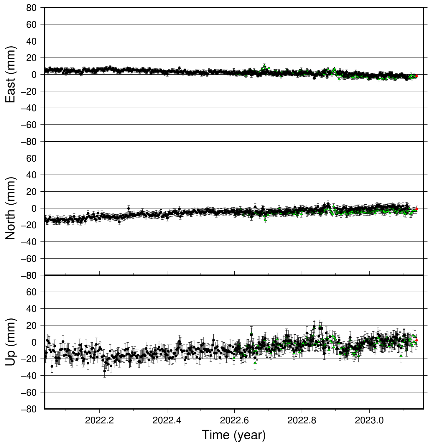
HAUD time series (IGS 2014), last 400 days
