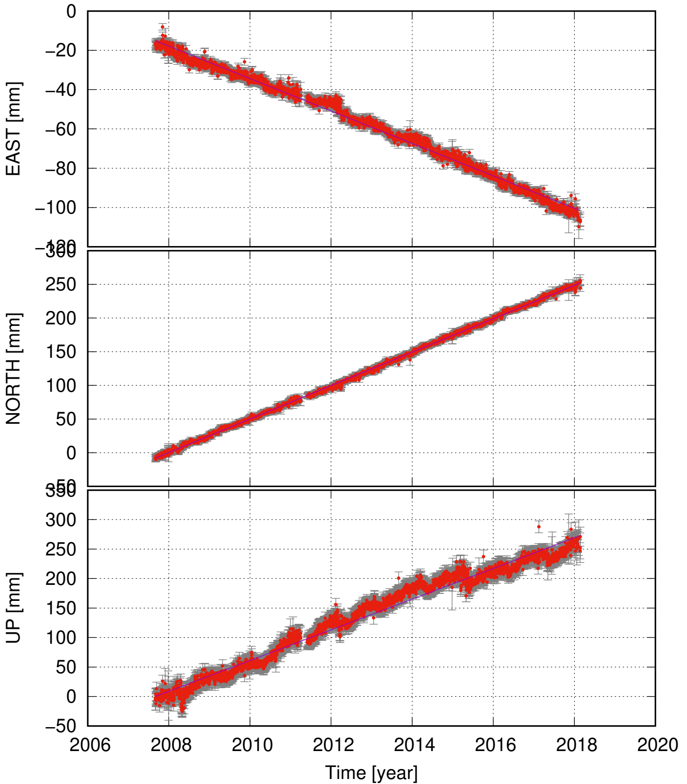
HAUC (64.71, -18.34) time series (ITRF 2014) v_e = -8.26 \pm 0.21 ; v_n = 24.81 \pm 0.20 ; v_u = 26.02 \pm 1.15 mm/yr
