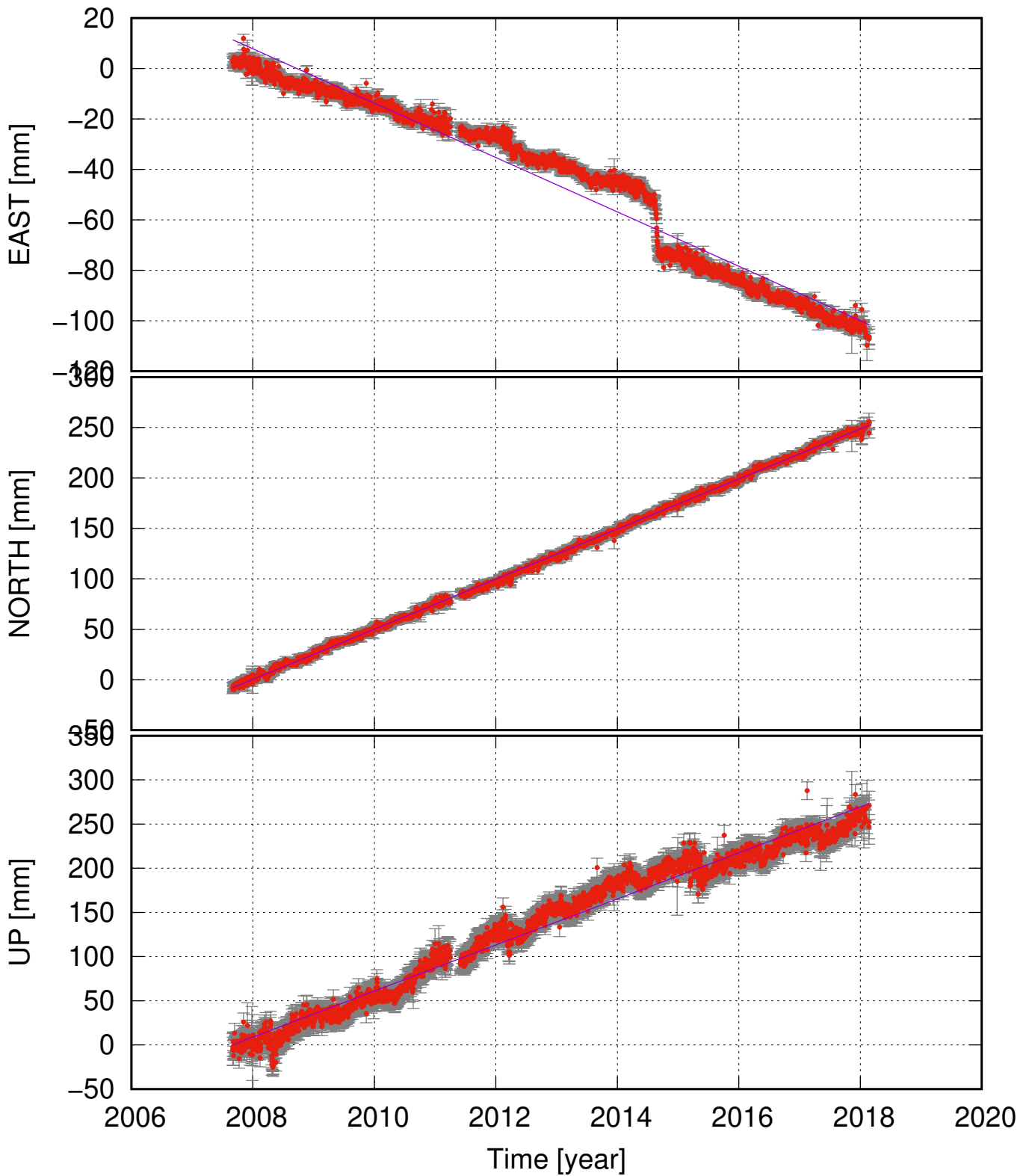
HAUC (64.71, -18.34) time series (ITRF 2014) v_e = -10.77 \pm 0.63 ; v_n = 24.81 \pm 0.20 ; v_u = 26.03 \pm 1.15 mm/yr
