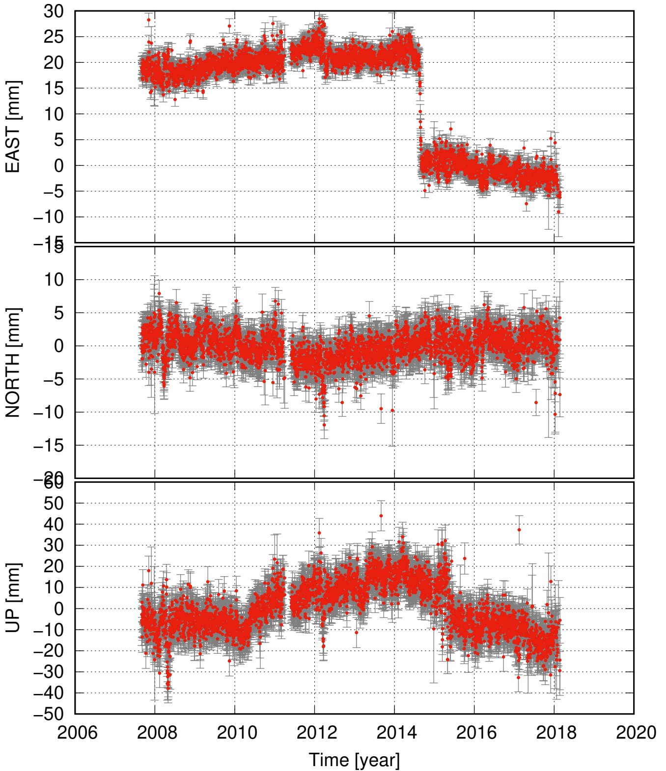
HAUC detrended and seasonal signal removed
