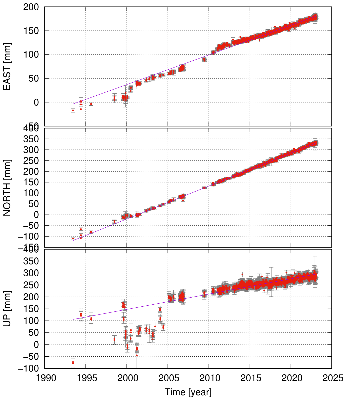
HAMR (63.62, -19.99) time series (ITRF 2014) v_e = 6.22 \pm 0.16 ; v_n = 15.21 \pm 0.10 ; v_u = 6.42 \pm 0.68 mm/yr
