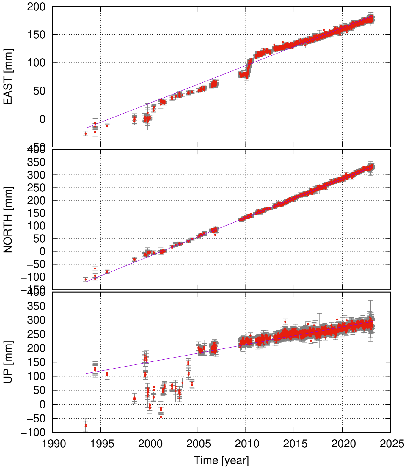
HAMR (63.62, -19.99) time series (ITRF 2014) v_e = 6.73 \pm 0.22 ; v_n = 15.21 \pm 0.10 ; v_u = 6.27 \pm 0.68 mm/yr
