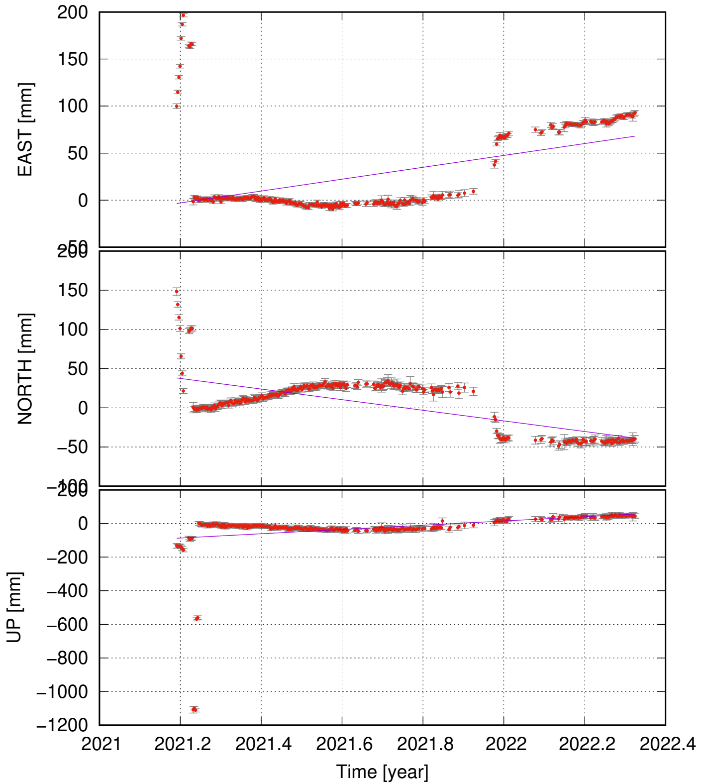
HAMD (63.86, -22.20) time series (ITRF 2014) v_e = 63.16 \pm 33.60 ; v_n = -67.72 \pm 20.87 ; v_u = 127.15 \pm 102.12 mm/yr
