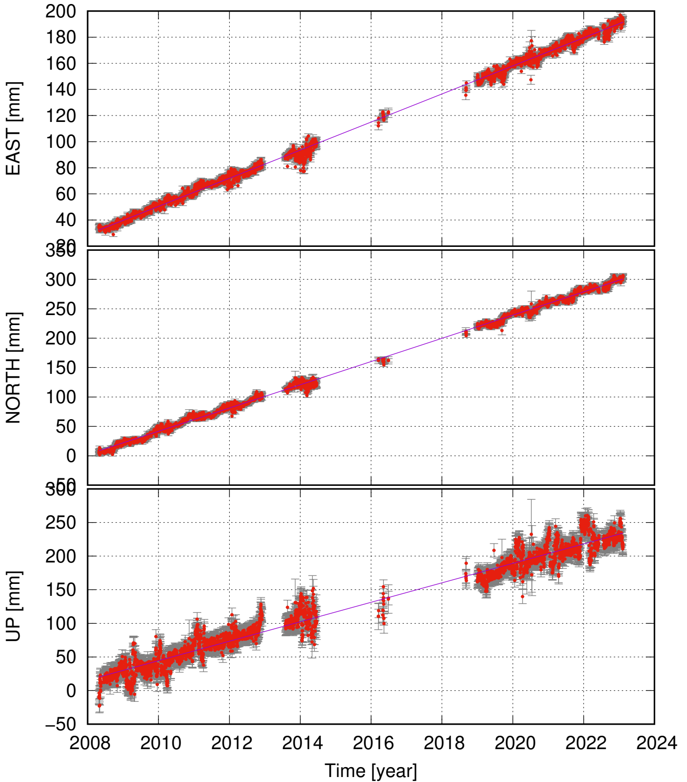
HAHV (64.95, -15.81) time series (ITRF 2014) v_e = 10.76 \pm 0.17 ; v_n = 19.76 \pm 0.29 ; v_u = 14.47 \pm 0.86 mm/yr
