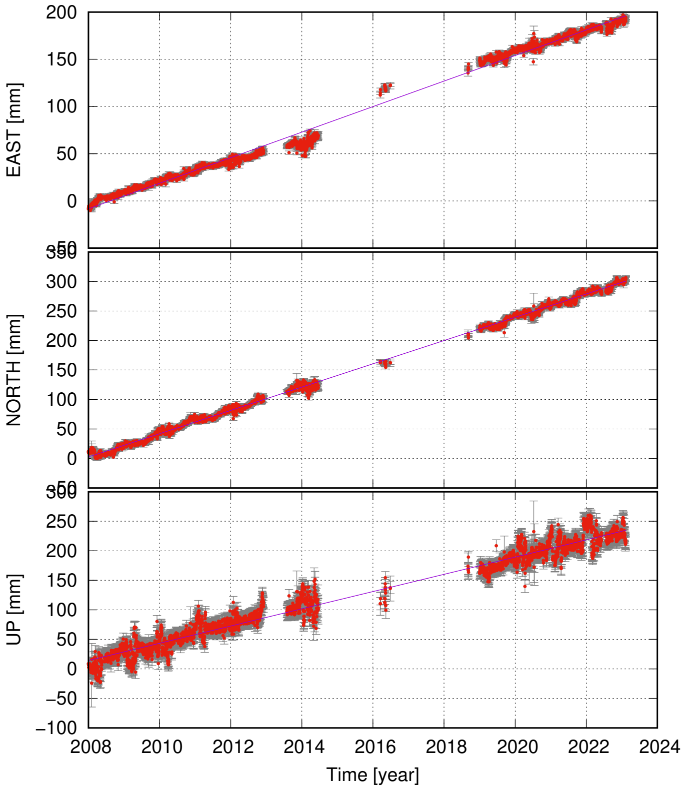
HAHV (64.95, -15.81) time series (ITRF 2014) ve = 13.53 ± 0.36; vn = 19.73 ± 0.29; vu = 14.60 ± 0.86 mm/yr
