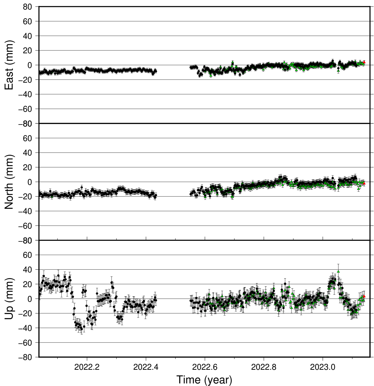
HAHV time series (IGS 2014), last 400 days
