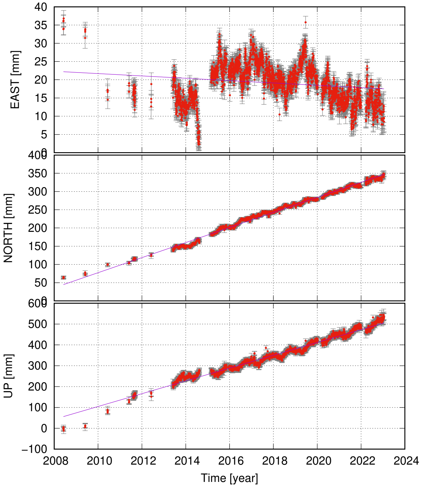
HAFS (64.48, -17.82) time series (ITRF 2014) v_e = -0.32 \pm 0.34 ; v_n = 20.66 \pm 0.40 ; v_u = 30.70 \pm 0.95 mm/yr
