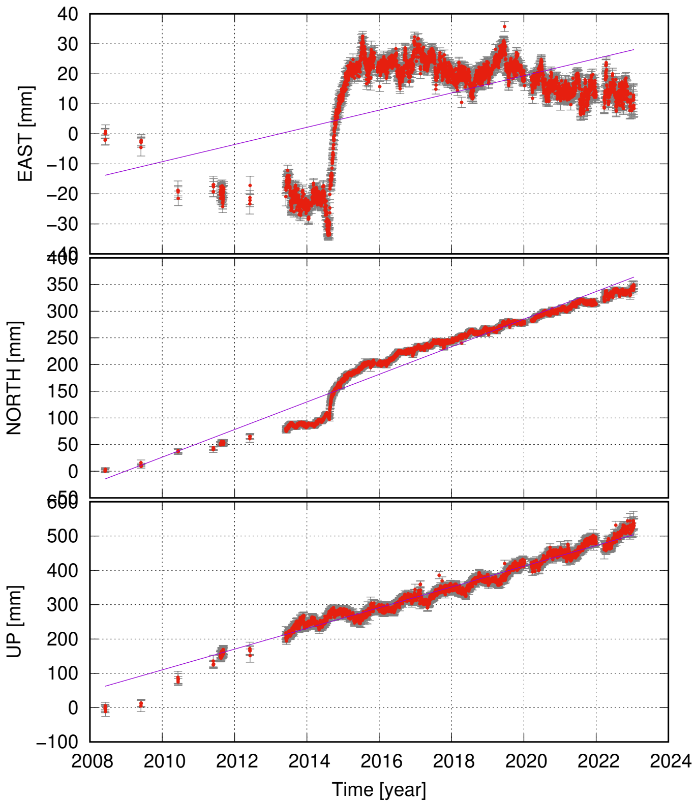
HAFS (64.48, -17.82) time series (ITRF 2014) v_e = 2.86 \pm 0.93 ; v_n = 25.88 \pm 1.41 ; v_u = 30.18 \pm 0.99 mm/yr
